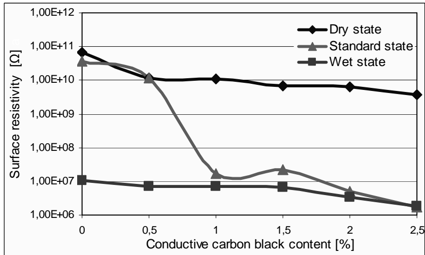
Picture 5. Surface resistance of samples containing conductive carbon.
