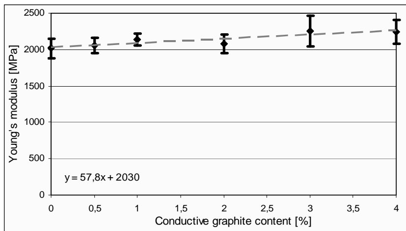
Figure 4. The Young's modulus of conductive graphite
