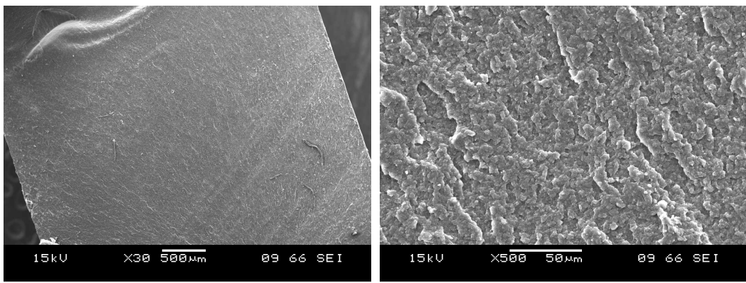
Figure 1. 30× and 500× enlarged SEM picture of 20% softening material
